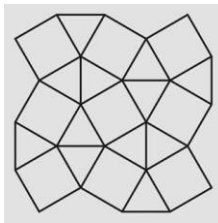
Figure 20: Tiling pattern 33434.
